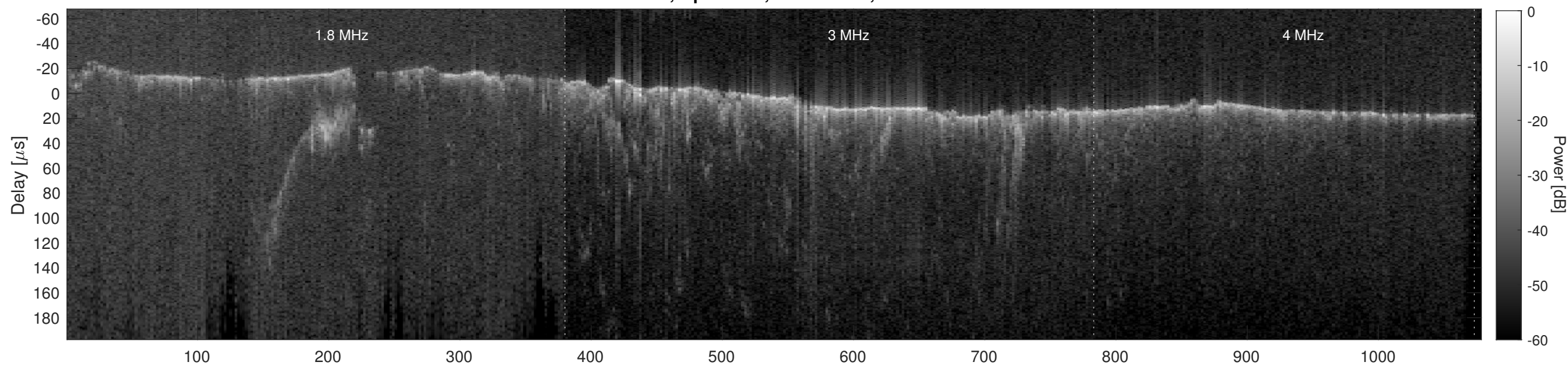
Orbit 8156, Cluttergram
