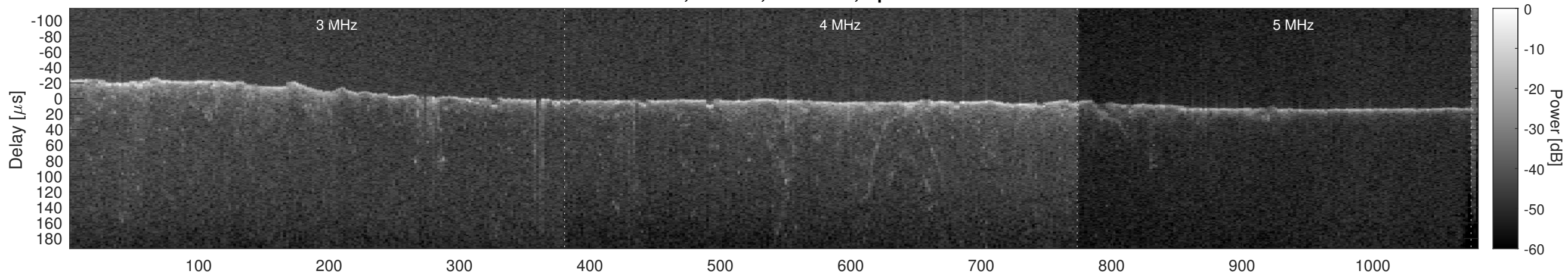
Orbit 8159, Cluttergram
