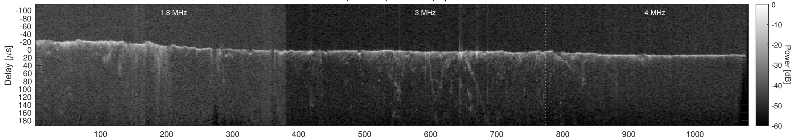
Orbit 8159, Cluttergram
