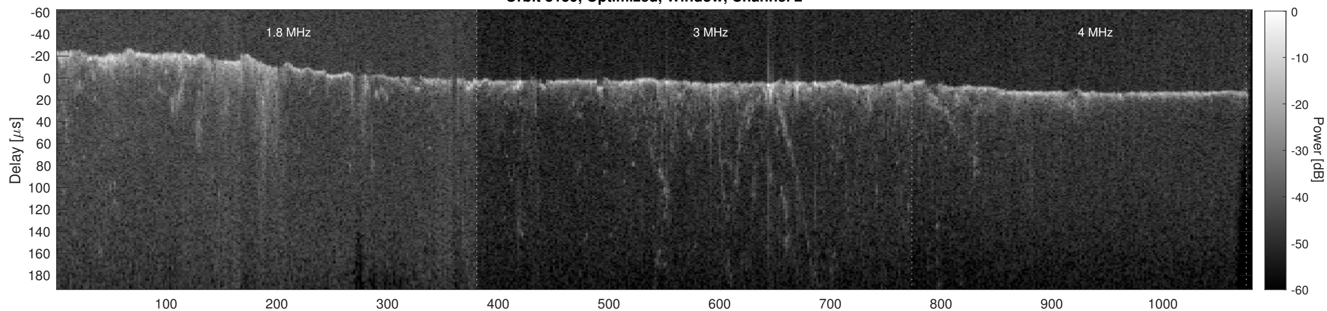
Orbit 8159, Cluttergram
