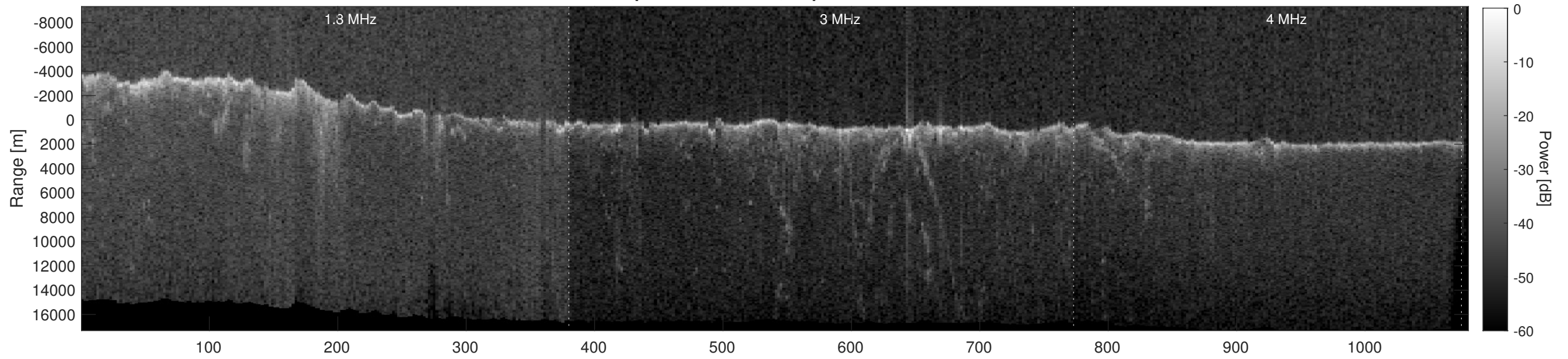
Orbit 8159, Depth-Corrected Cluttergram
