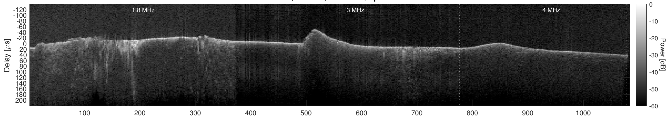
Orbit 8160, Cluttergram
