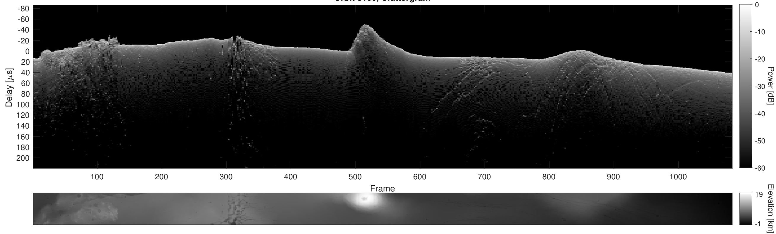
Orbit 8160, Cluttergram
