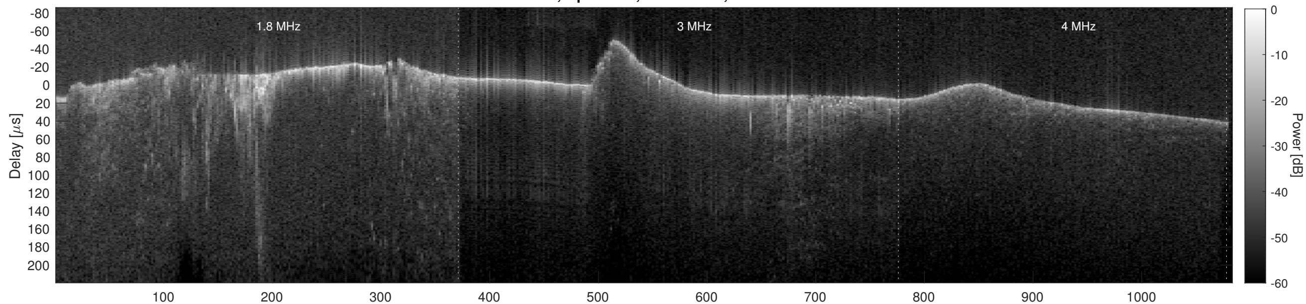
Orbit 8160, Cluttergram
