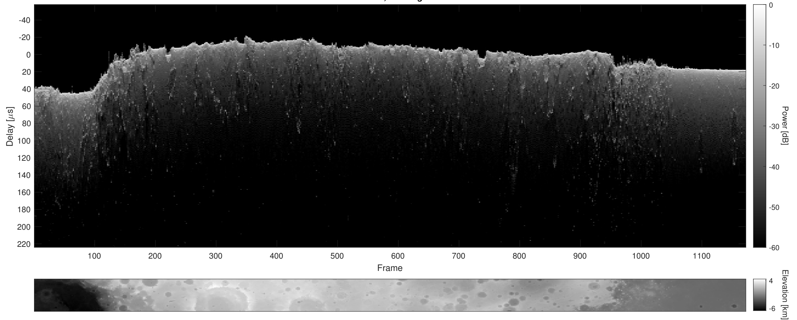
Orbit 8162, Cluttergram
