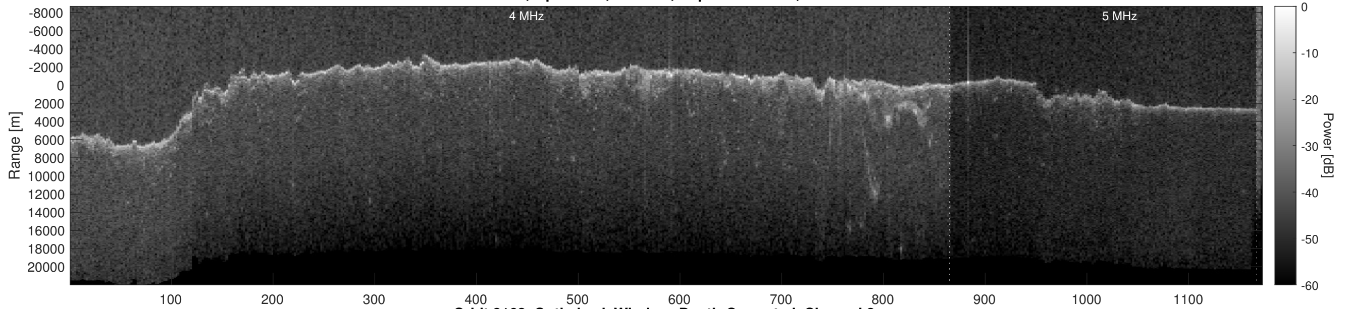
Orbit 8162, Optimized, Window, Depth-Corrected, Channel 2
