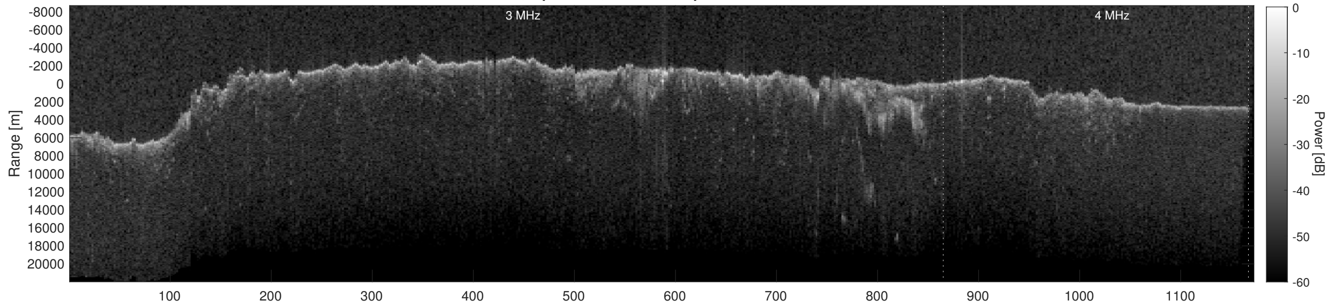
Orbit 8162, Depth-Corrected Cluttergram
