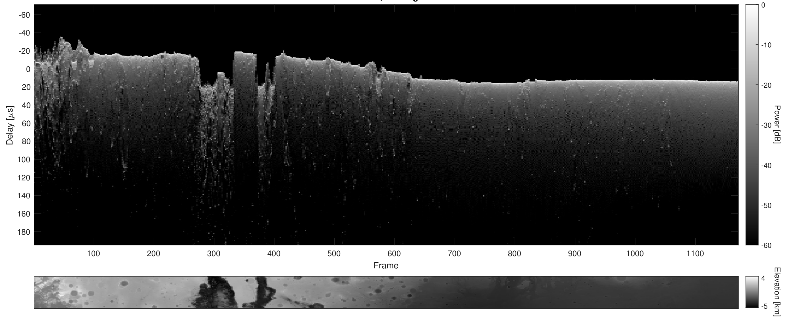
Orbit 8163, Cluttergram
