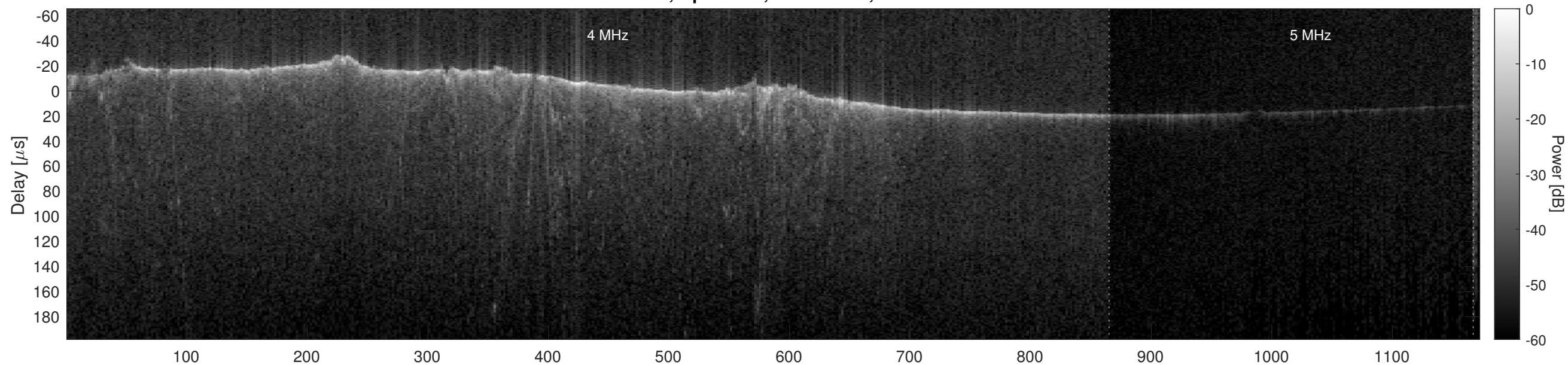
Orbit 8165, Optimized, No Window, Channel 2
