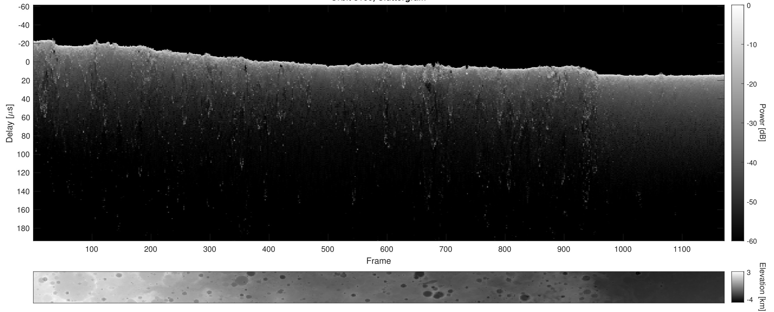
Orbit 8166, Cluttergram
