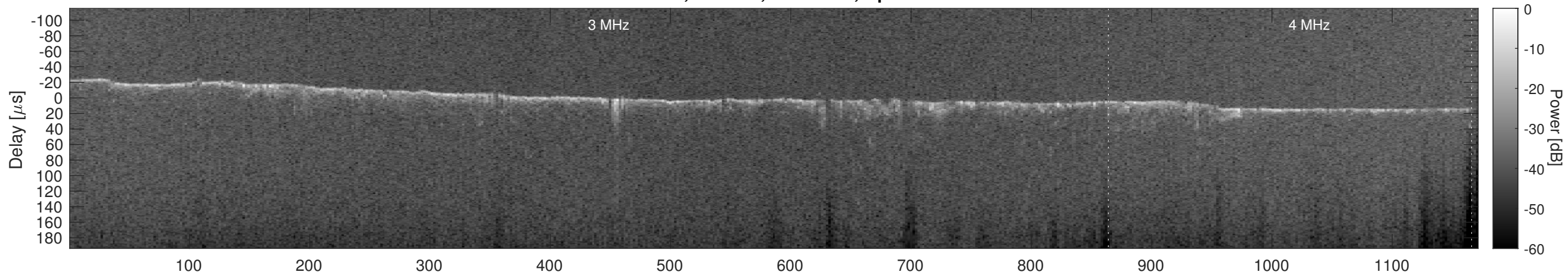
Orbit 8166, Cluttergram
