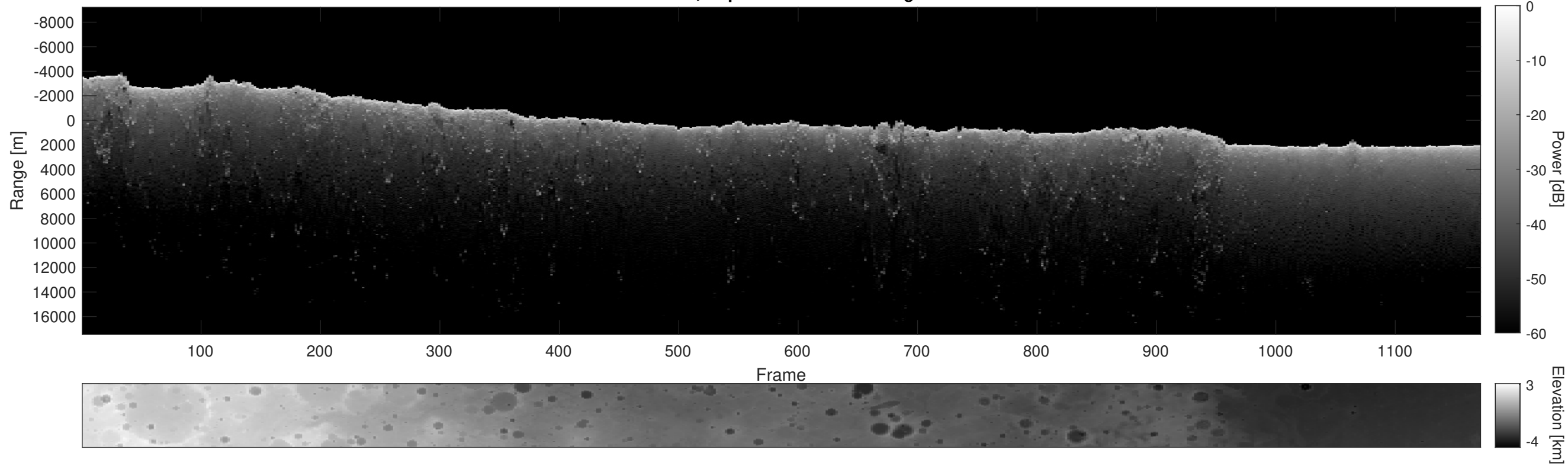
Orbit 8166, Depth-Corrected Cluttergram
