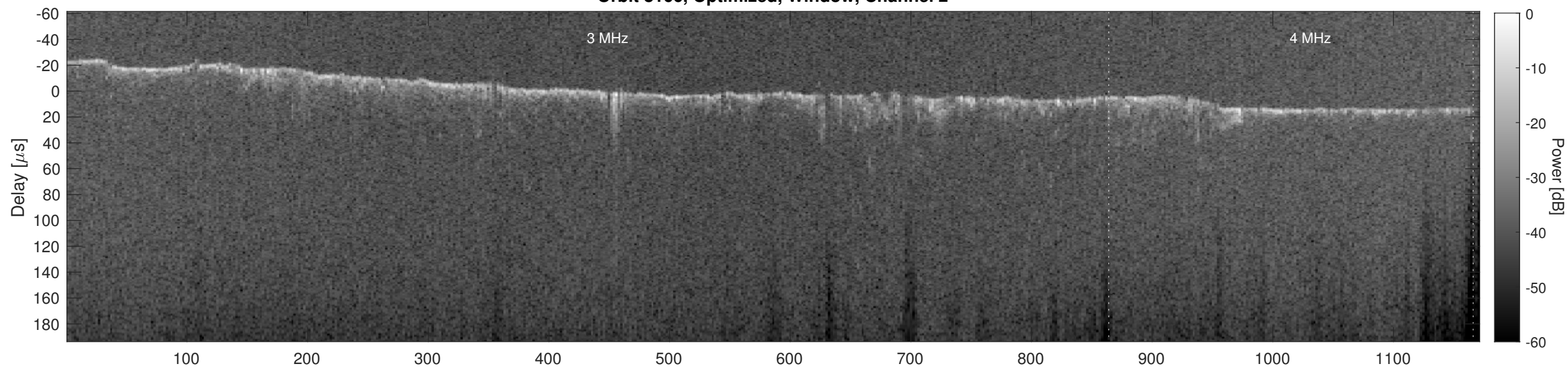
Orbit 8166, Cluttergram
