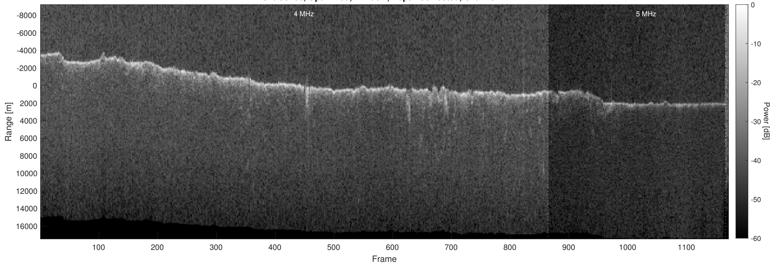
Orbit 8166, Optimized, Window, Depth-Corrected, Channel 2
