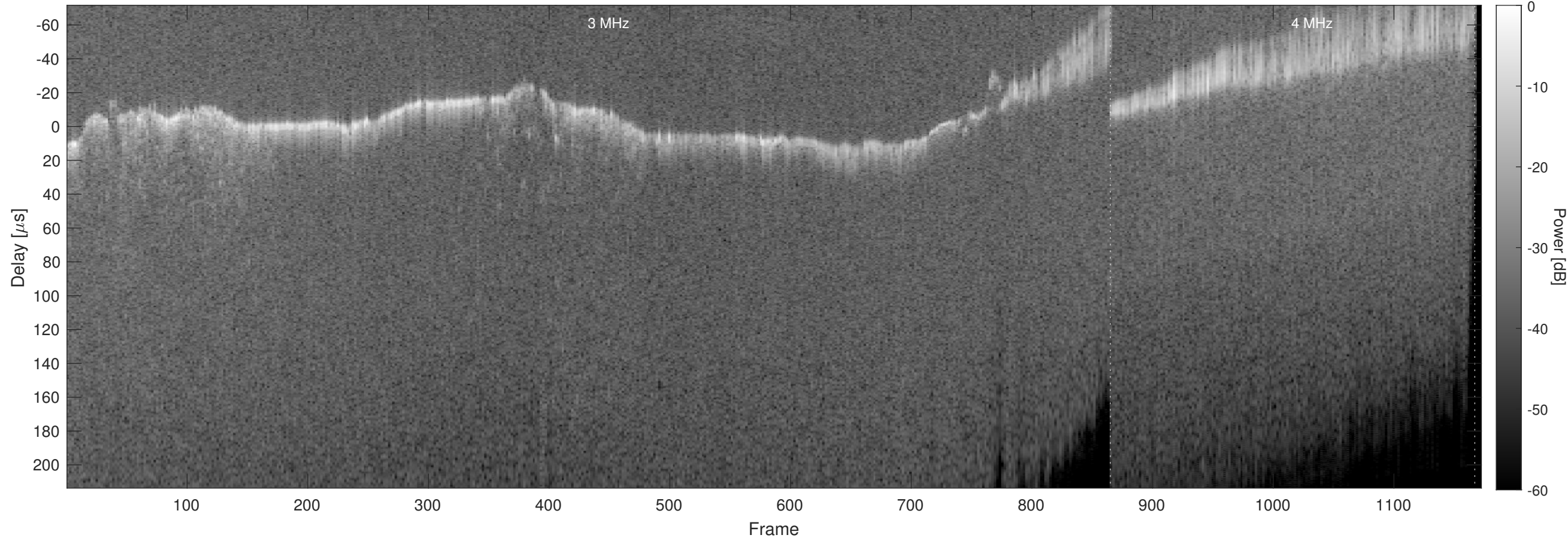
Orbit 8167, Chapman, No Window, Channel 2
