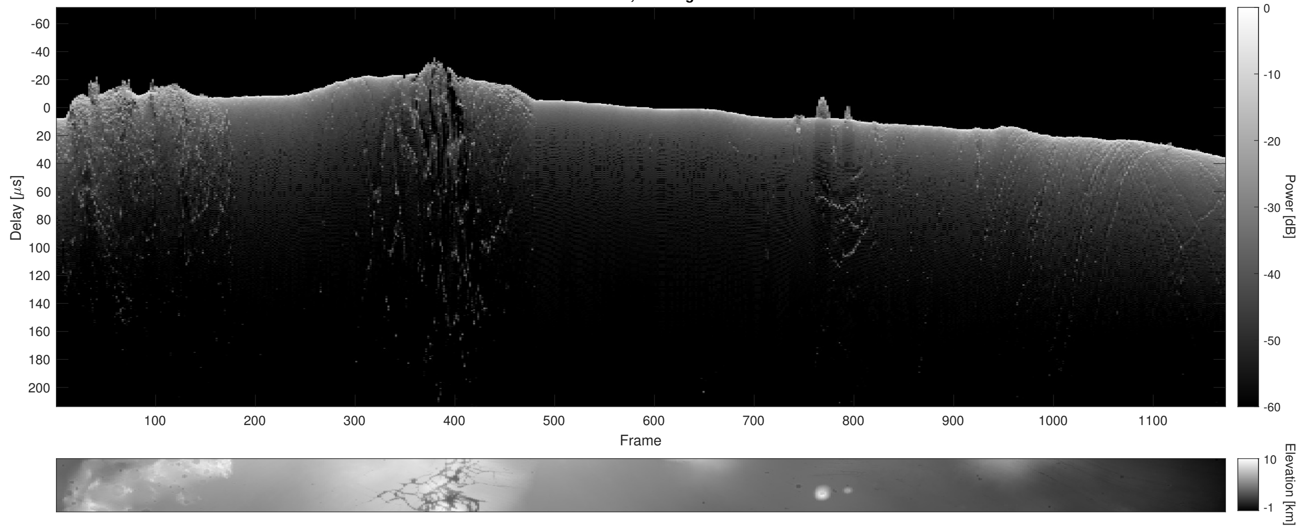
Orbit 8167, Cluttergram
