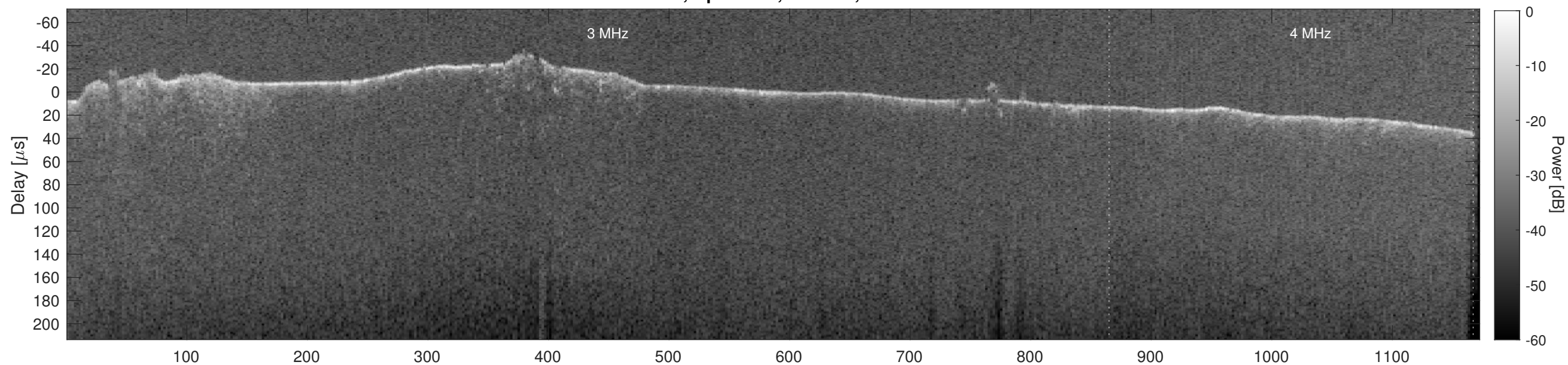
Orbit 8167, Cluttergram
