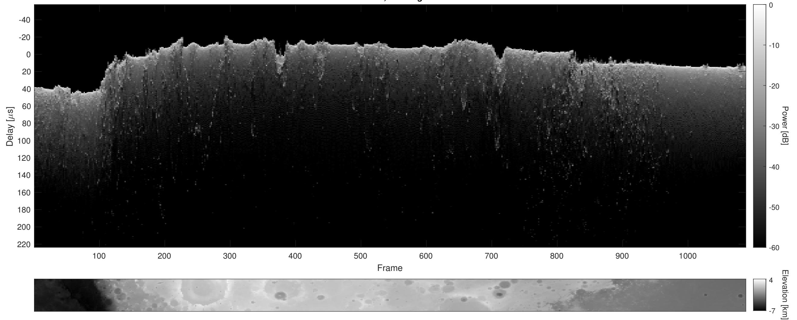
Orbit 8169, Cluttergram
