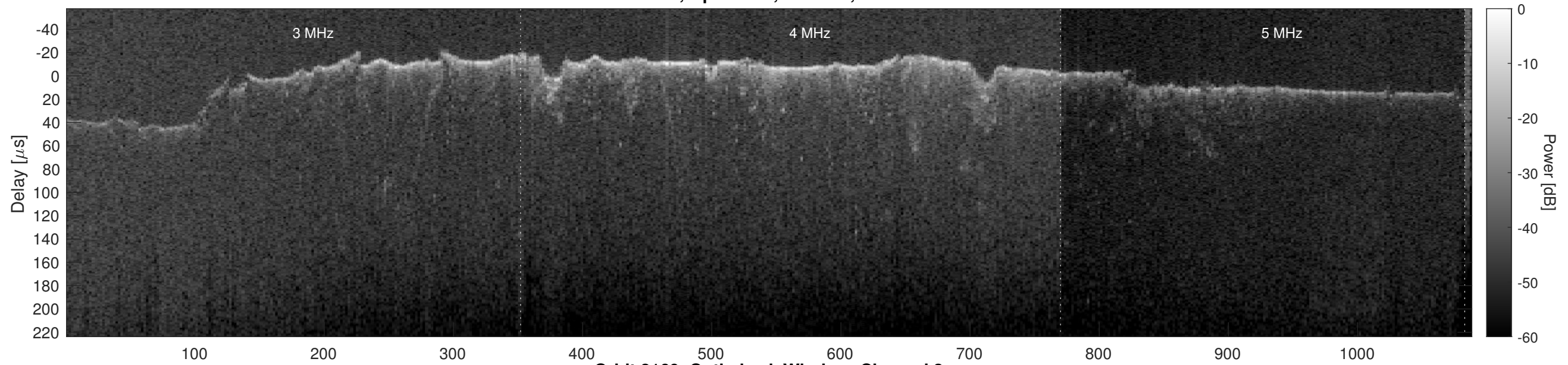
Orbit 8169, Optimized, Window, Channel 2
