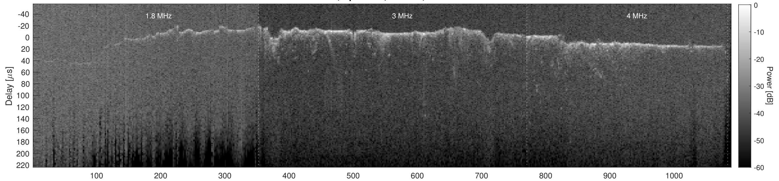
Orbit 8169, Cluttergram
