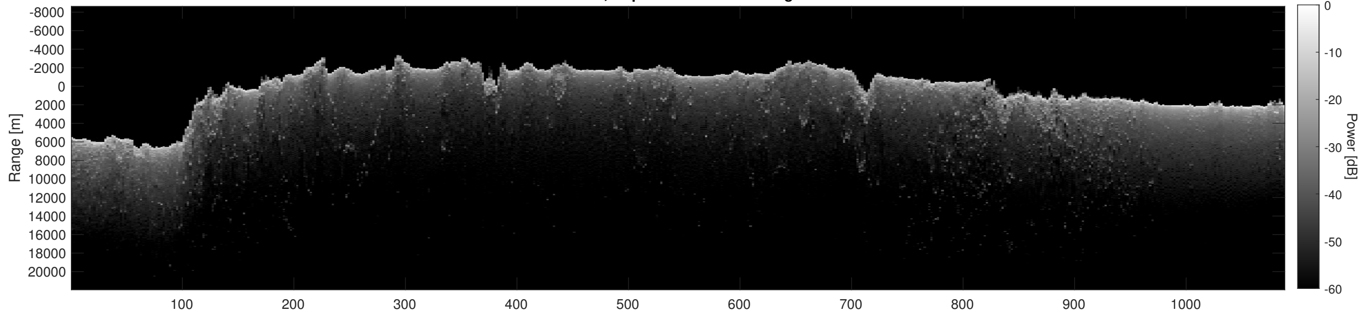
Orbit 8169, Depth-Corrected Cluttergram
