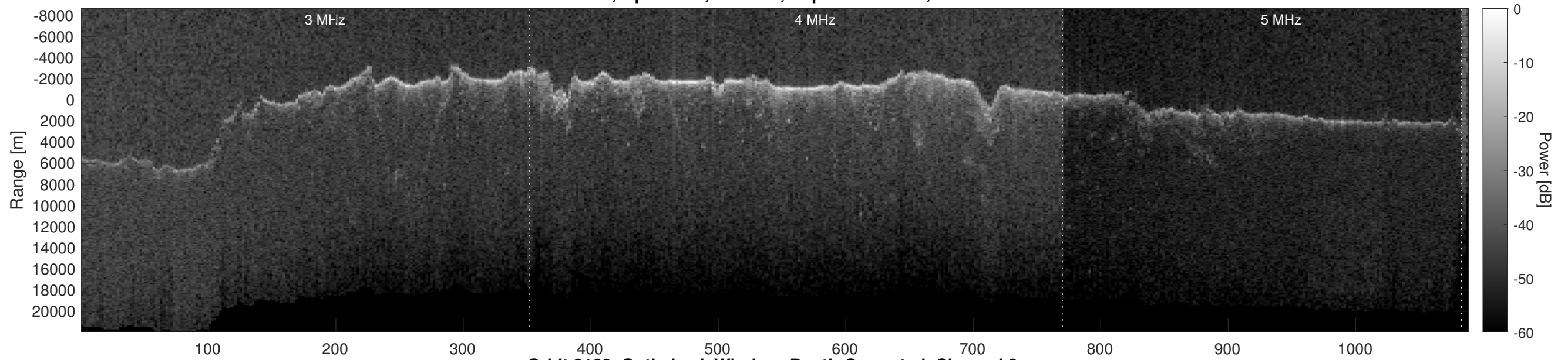
Orbit 8169, Optimized, Window, Depth-Corrected, Channel 2
