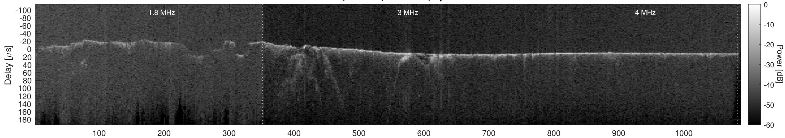
Orbit 8170, Cluttergram
