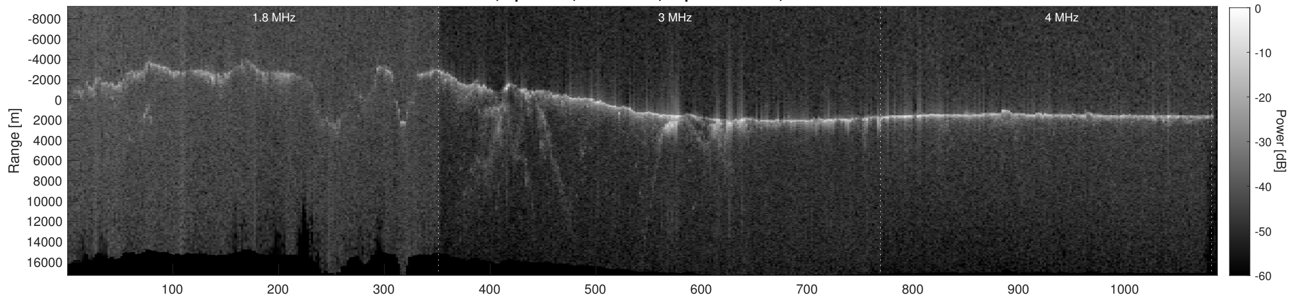
Orbit 8170, Depth-Corrected Cluttergram
