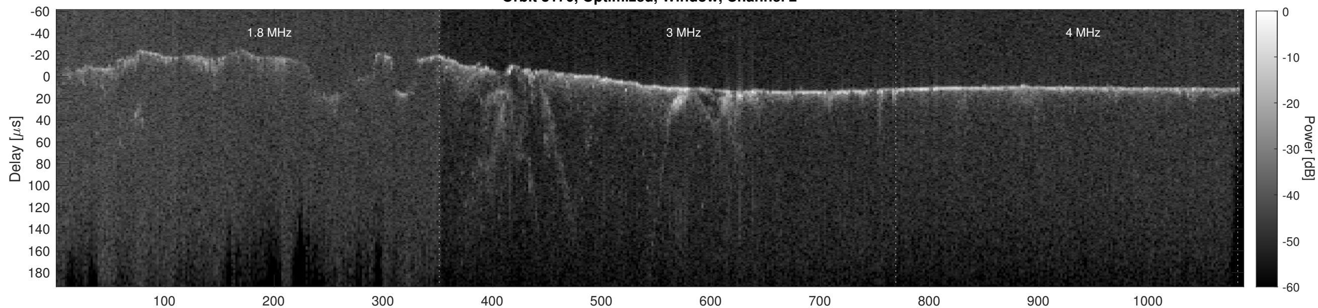
Orbit 8170, Cluttergram
