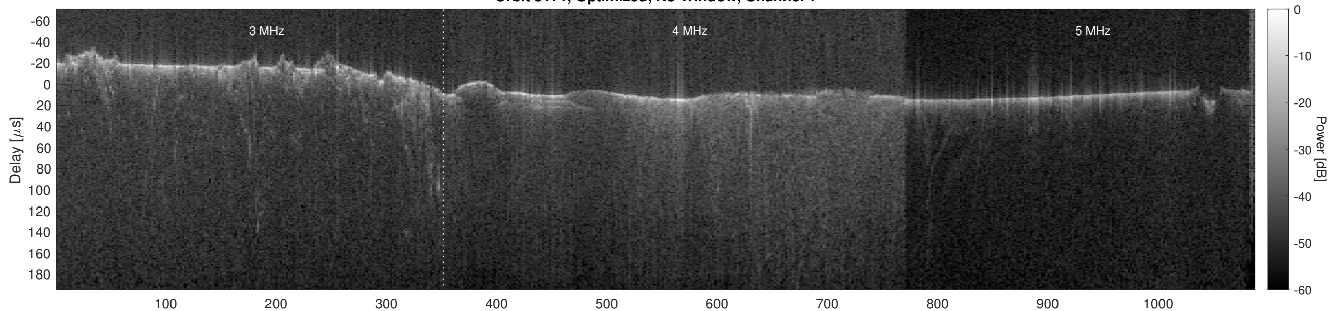
Orbit 8171, Optimized, No Window, Channel 2
