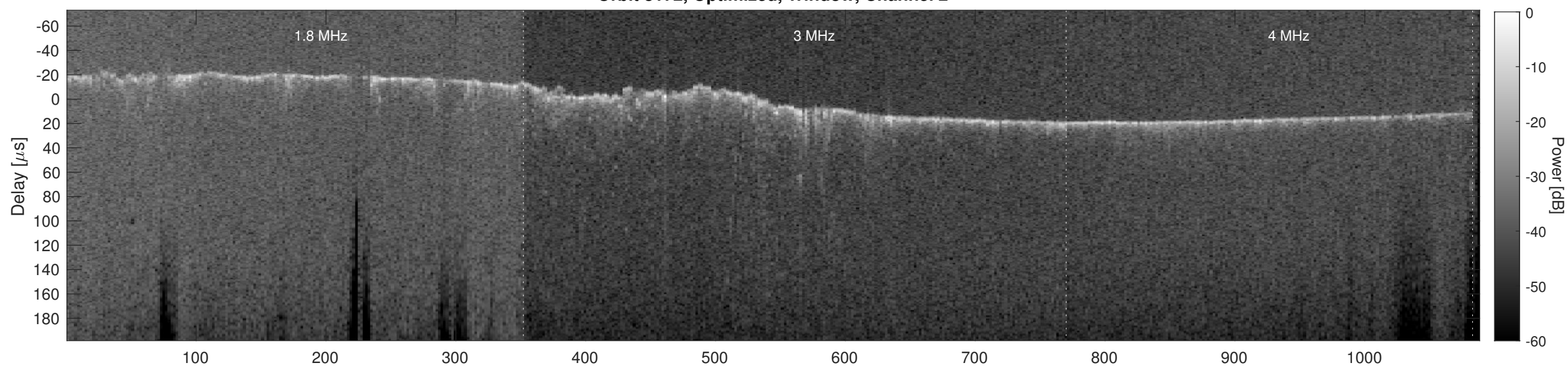
Orbit 8172, Cluttergram
