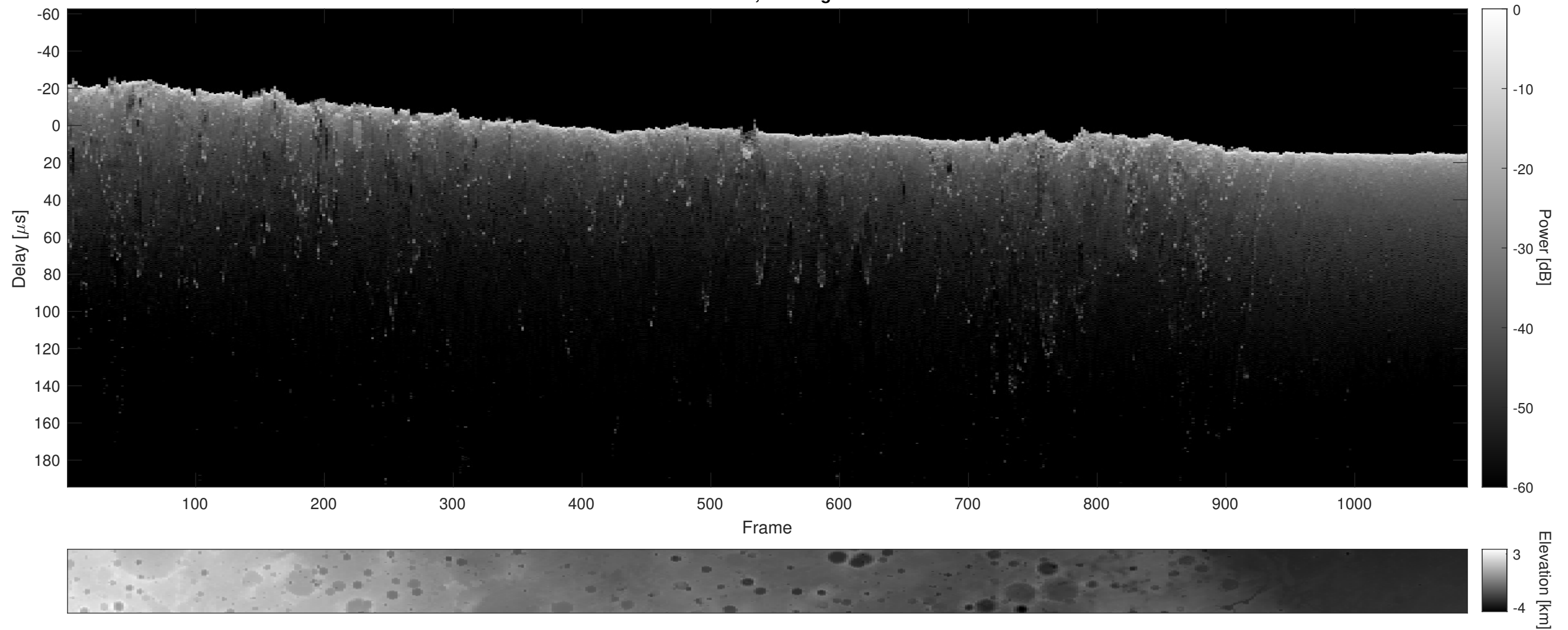
Orbit 8173, Cluttergram
