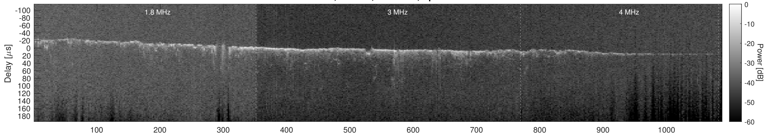
Orbit 8173, Cluttergram
