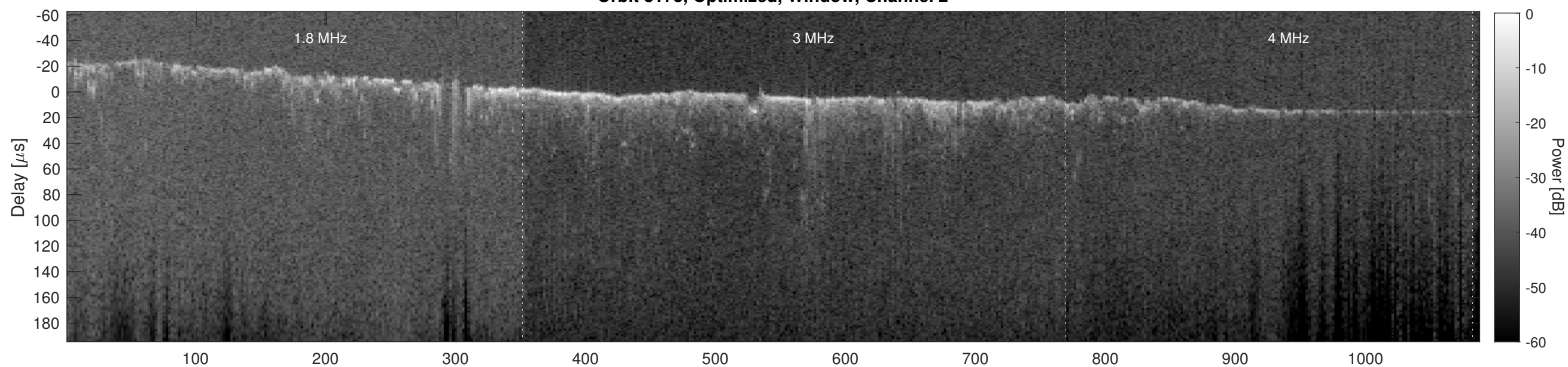
Orbit 8173, Cluttergram
