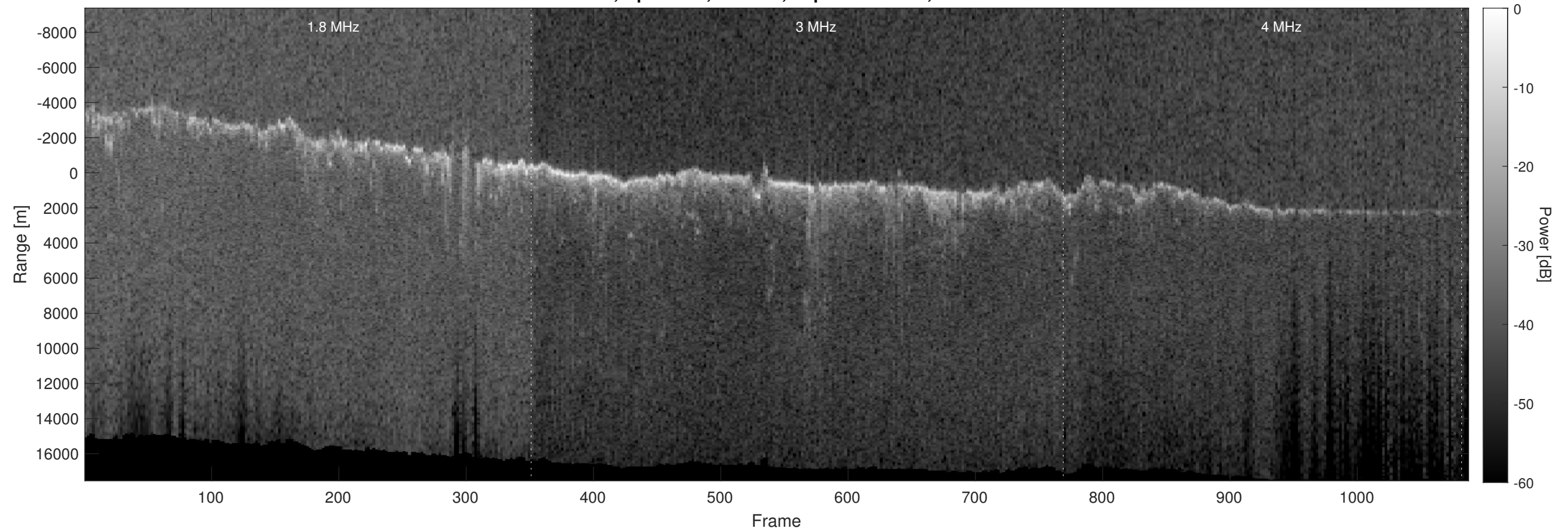
Orbit 8173, Optimized, Window, Depth-Corrected, Channel 2
