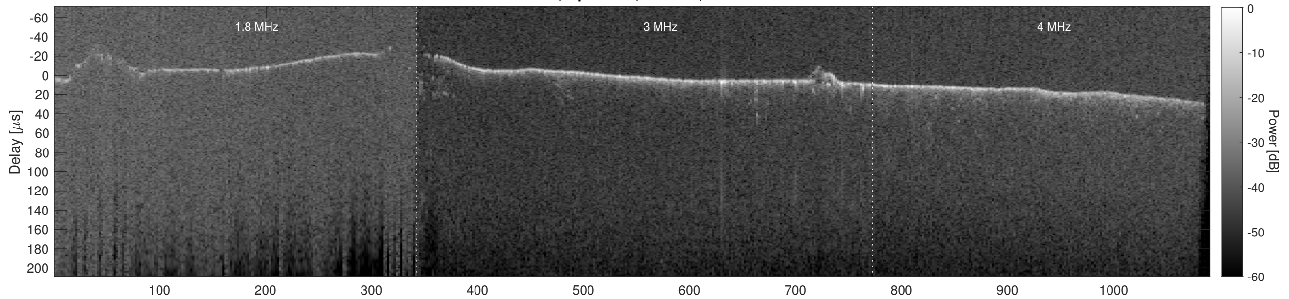
Orbit 8174, Cluttergram
