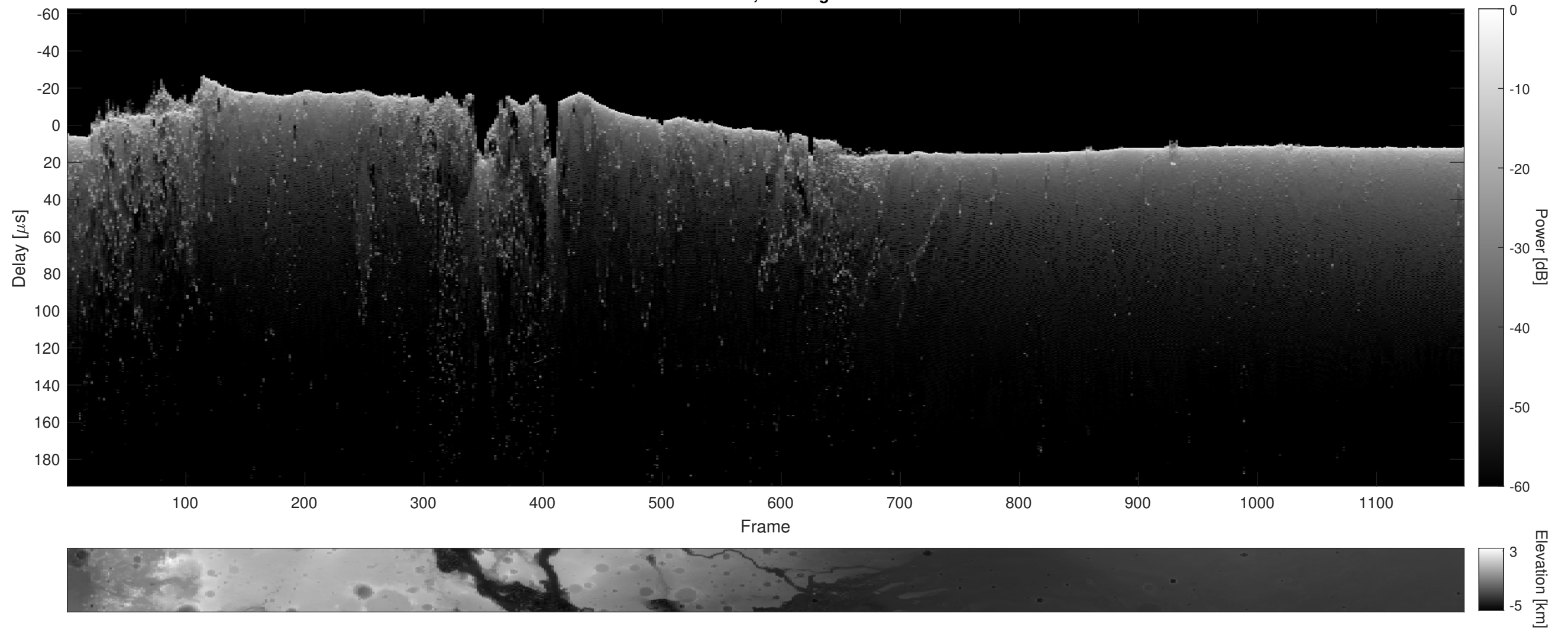
Orbit 8177, Cluttergram
