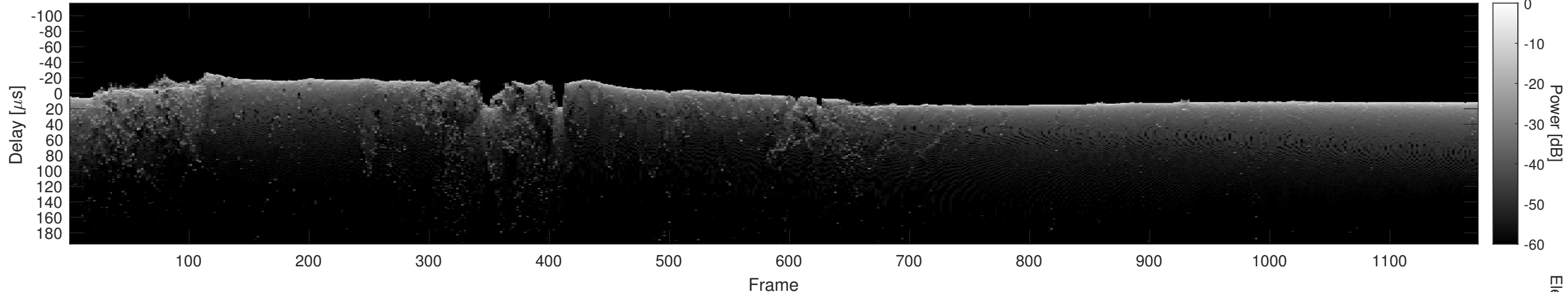
Orbit 8177, Cluttergram
