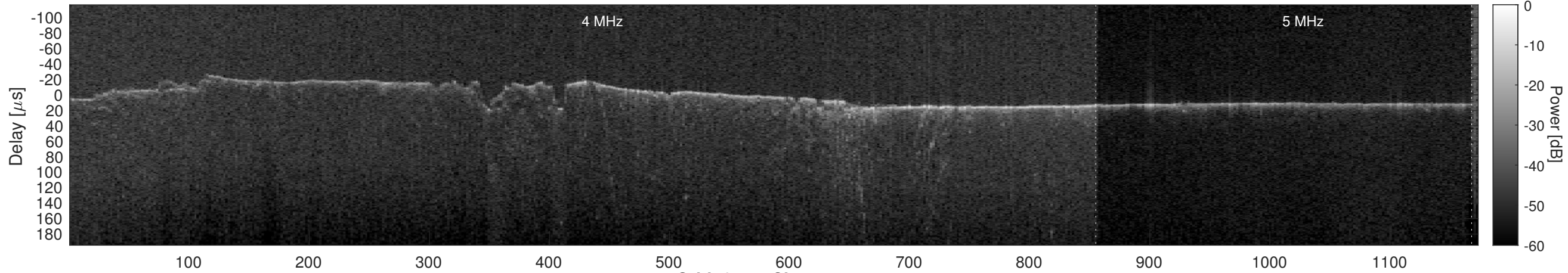
Orbit 8177, Cluttergram
