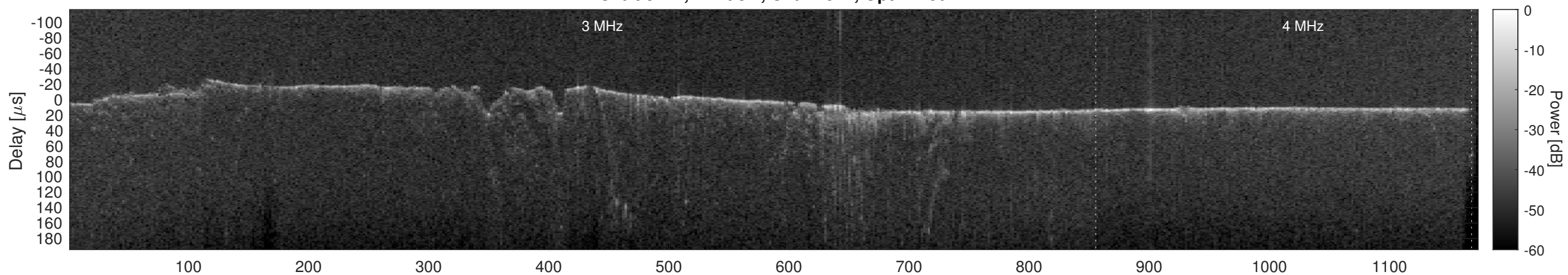
Orbit 8177, Cluttergram
