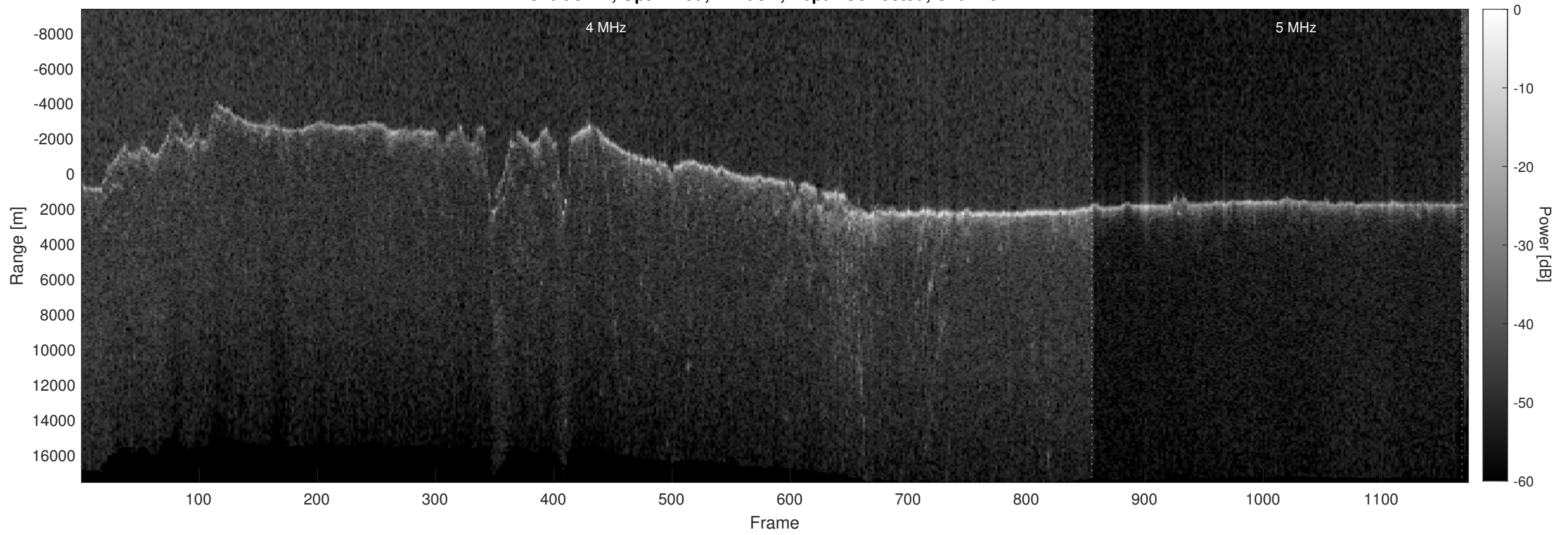
Orbit 8177, Optimized, Window, Depth-Corrected, Channel 2
