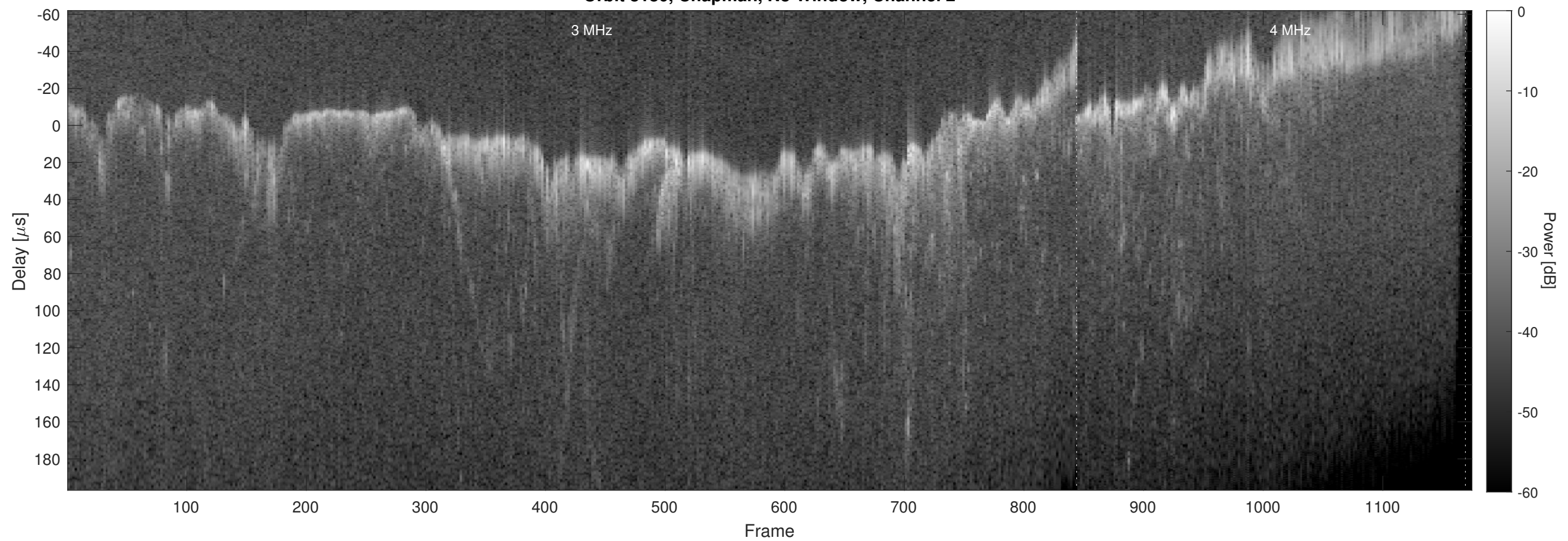
Orbit 8180, Chapman, No Window, Channel 2
