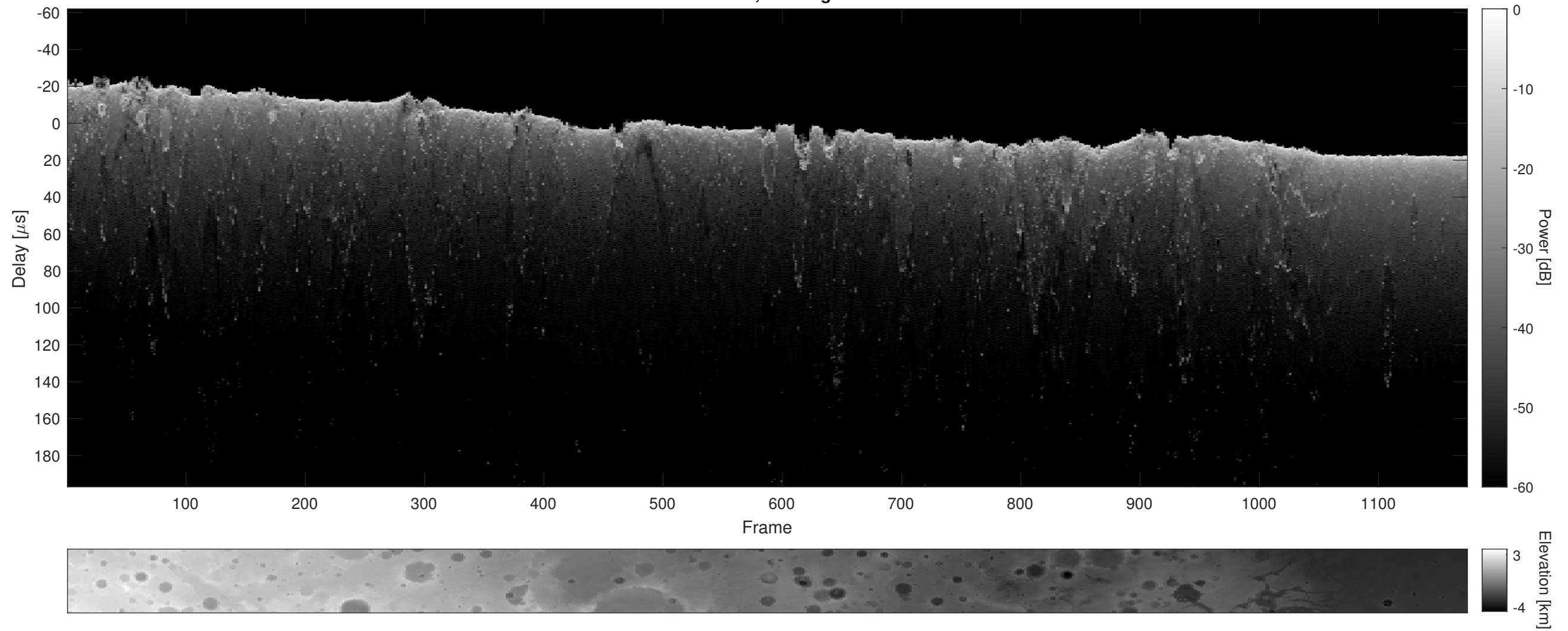
Orbit 8180, Cluttergram
