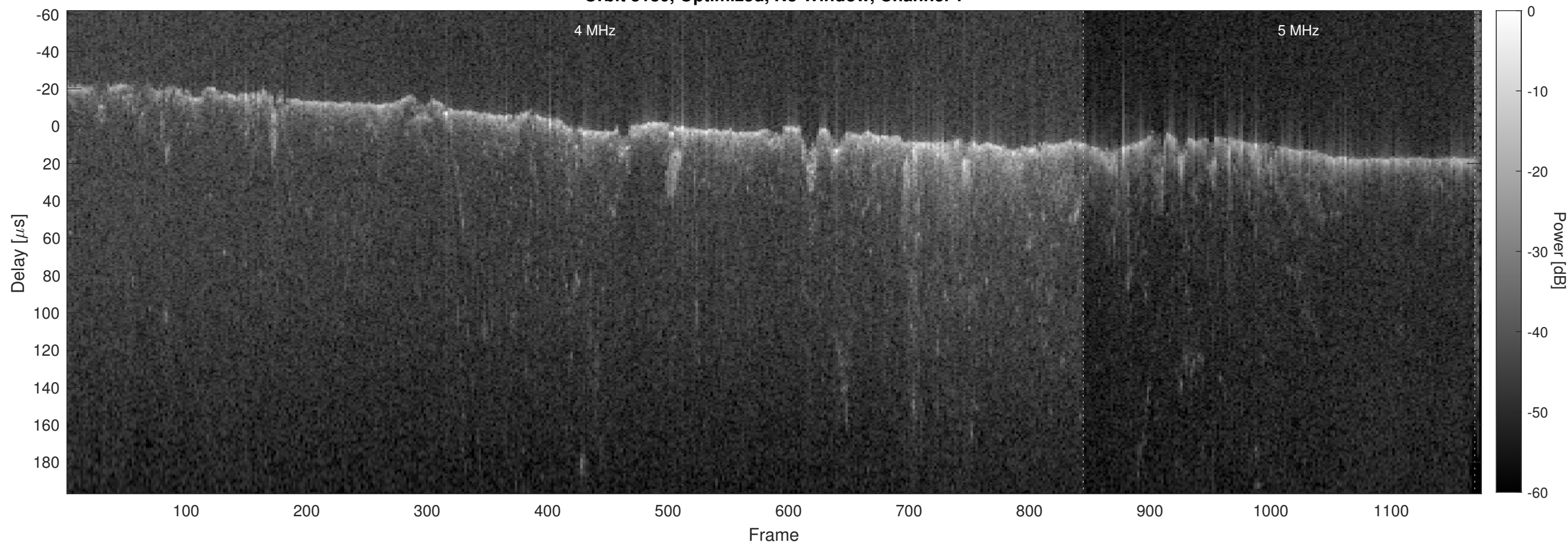
Orbit 8180, Optimized, No Window, Channel 2
