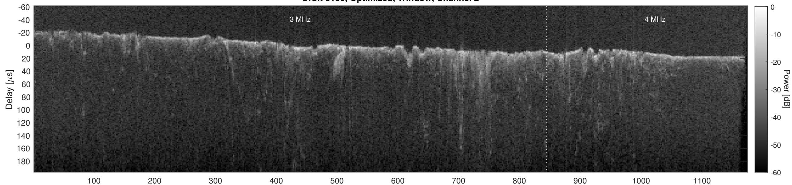
Orbit 8180, Cluttergram
