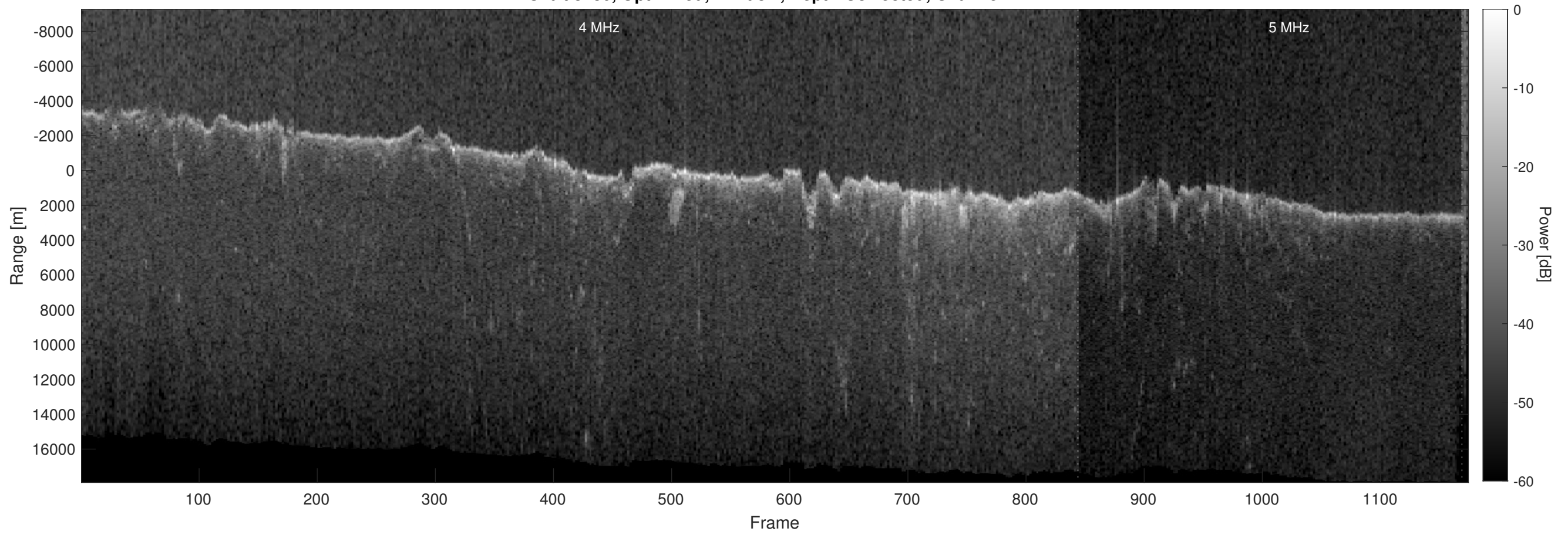
Orbit 8180, Optimized, Window, Depth-Corrected, Channel 2
