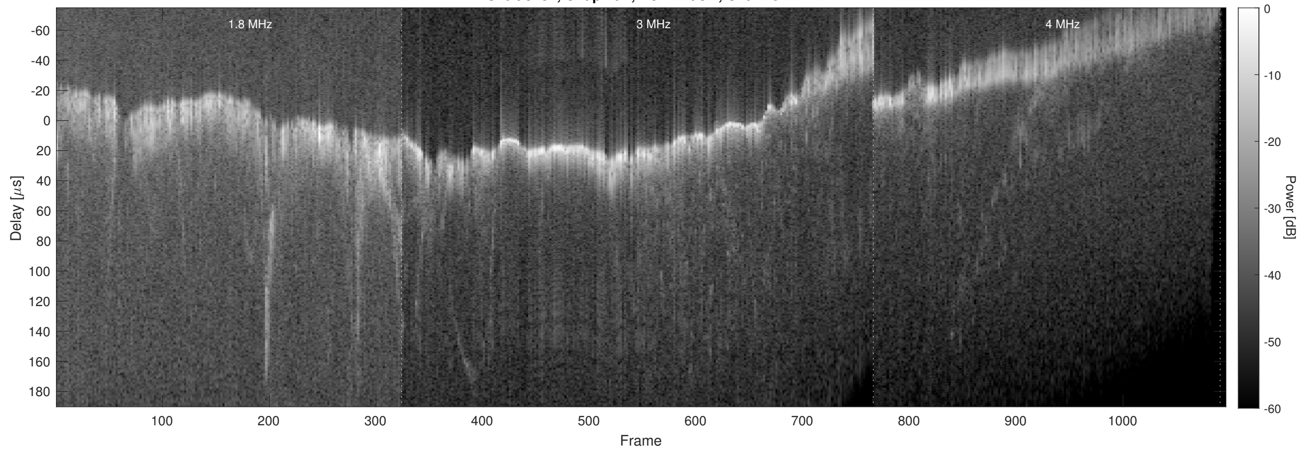
Orbit 8182, Chapman, No Window, Channel 2
