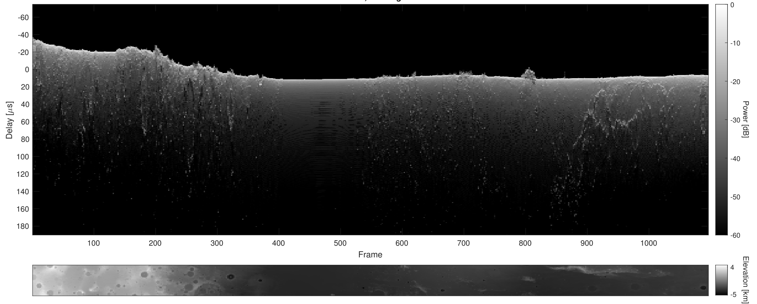
Orbit 8182, Cluttergram
