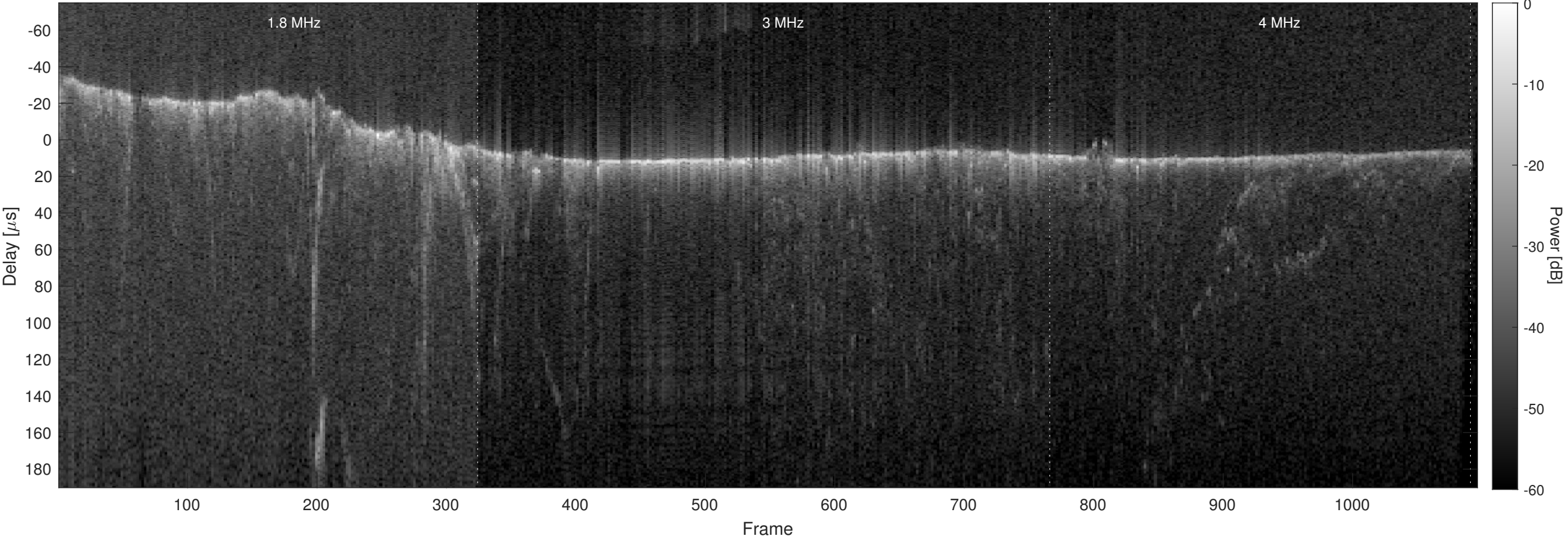
Orbit 8182, Optimized, No Window, Channel 2
