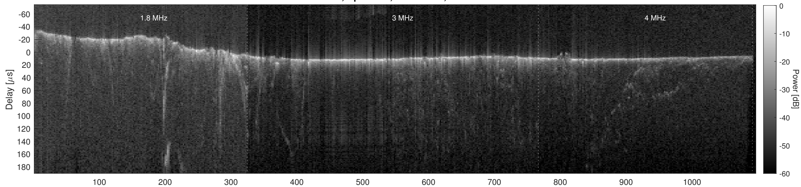
Orbit 8182, Cluttergram
