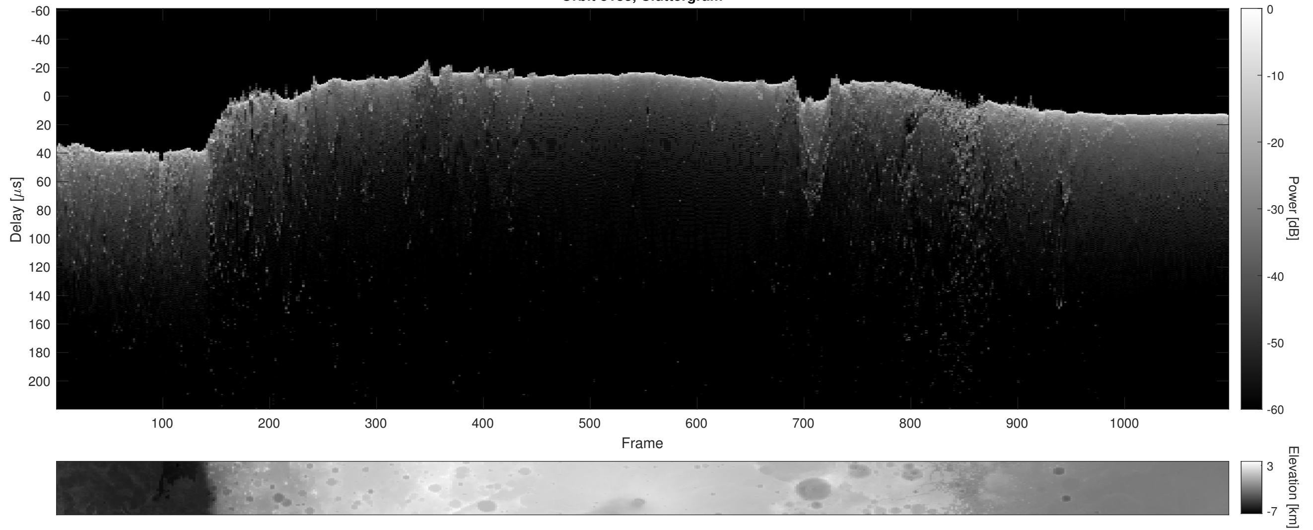
Orbit 8183, Cluttergram
