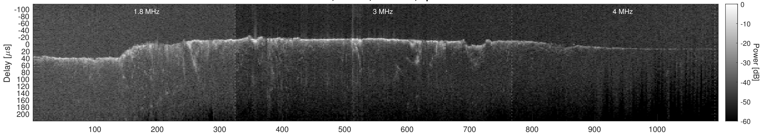
Orbit 8183, Cluttergram
