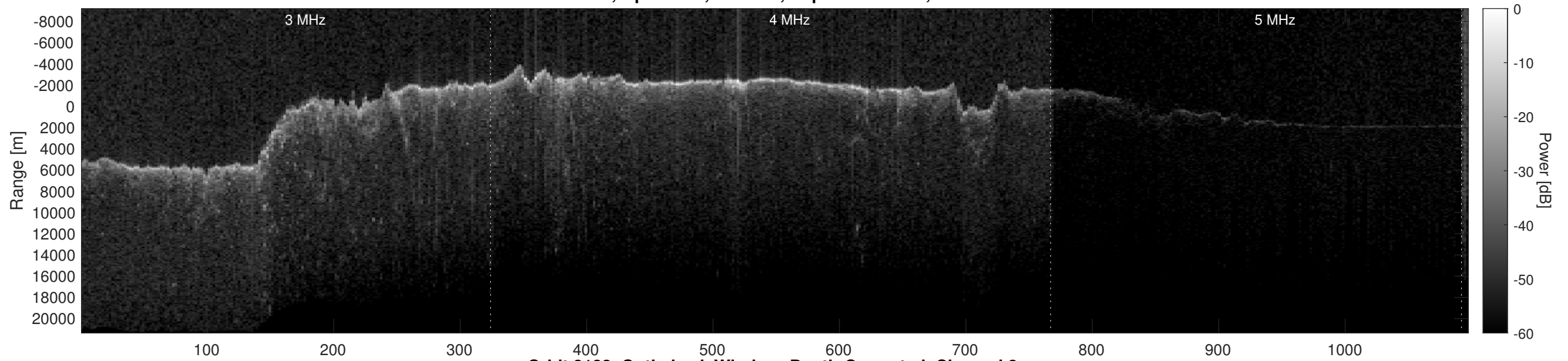
Orbit 8183, Optimized, Window, Depth-Corrected, Channel 2
