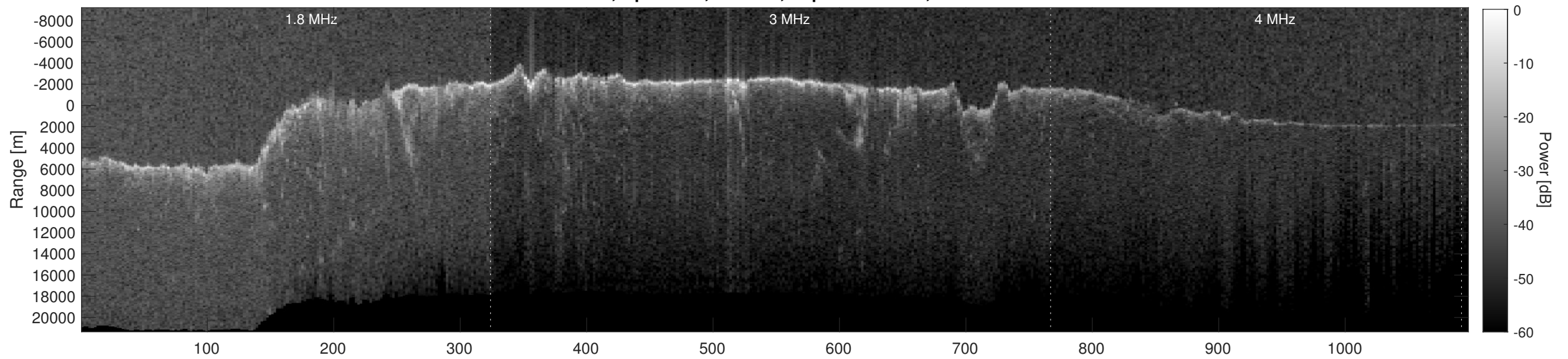
Orbit 8183, Depth-Corrected Cluttergram
