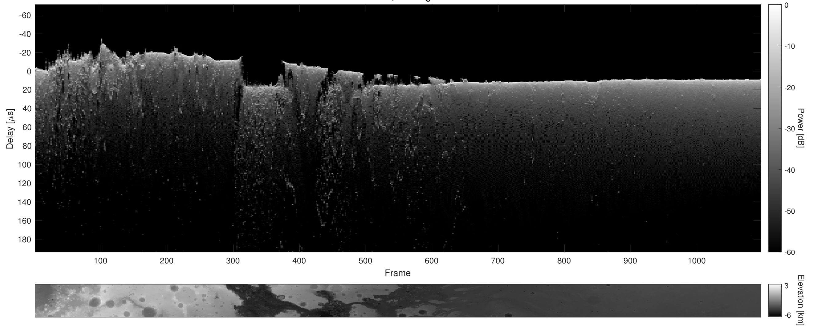
Orbit 8184, Cluttergram
