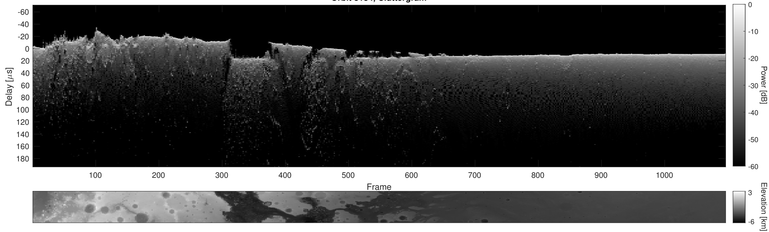
Orbit 8184, Cluttergram
